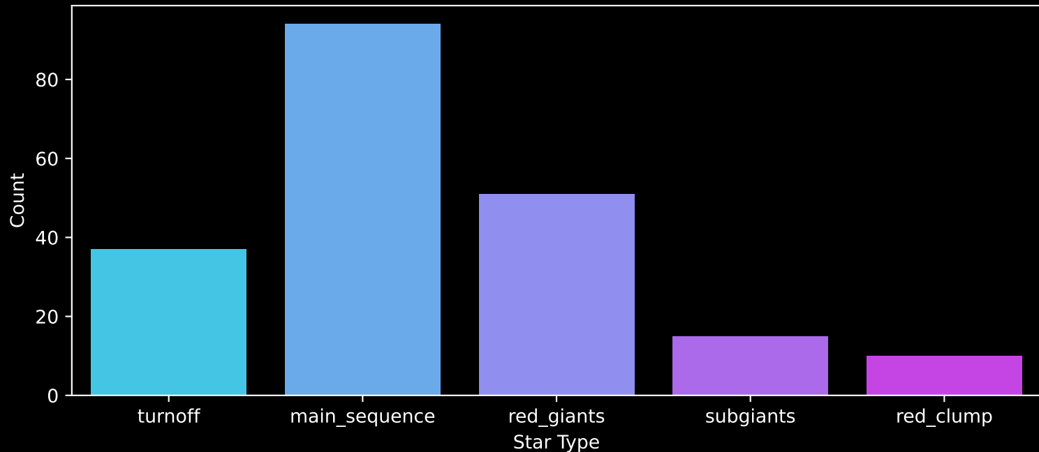
APOGEE DR17 Field: [184+31] Count plot of Star Type
