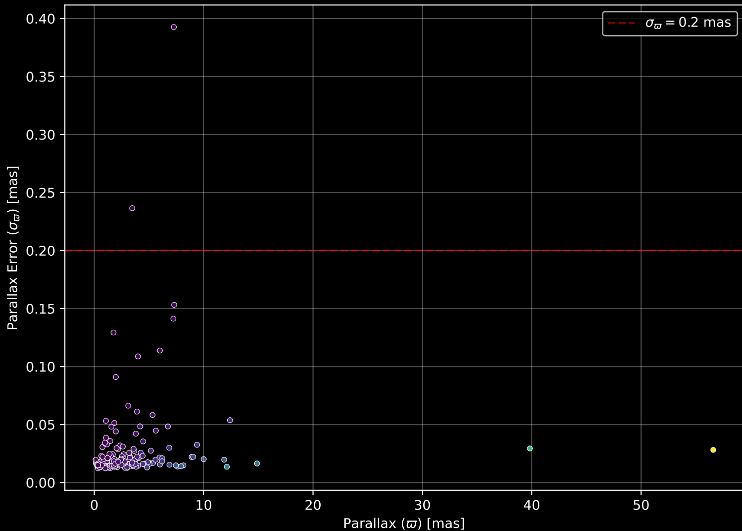
APOGEE DR17 Field: [184+31] Parallax Quality (n= 207)
