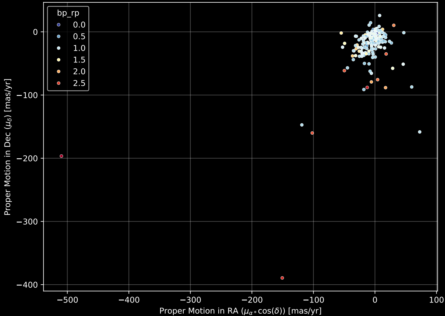
APOGEE DR17 Field: [184+31] Proper Motion Diagram (n= 207)
