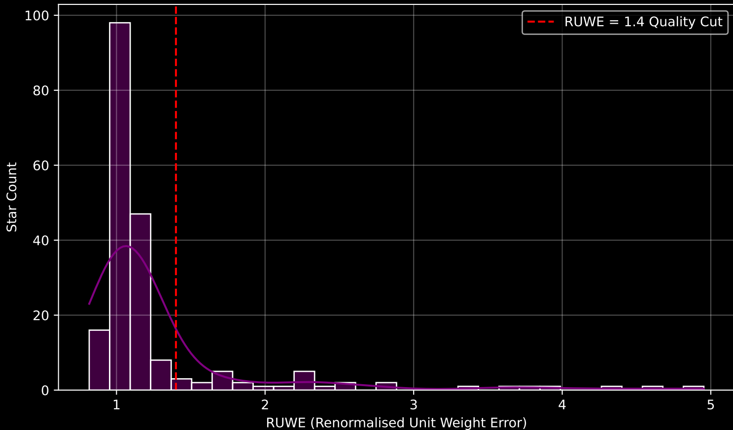
GAPOGEE DR17 Field [184+31] RUWE Distribution (n= 200)
