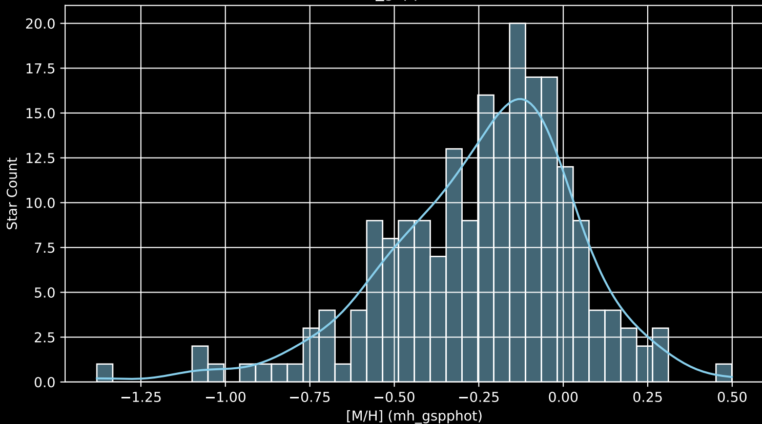
APOGEE DR17 Field: [184+31 [M/H] (mh_gspphot) (n= 207)
