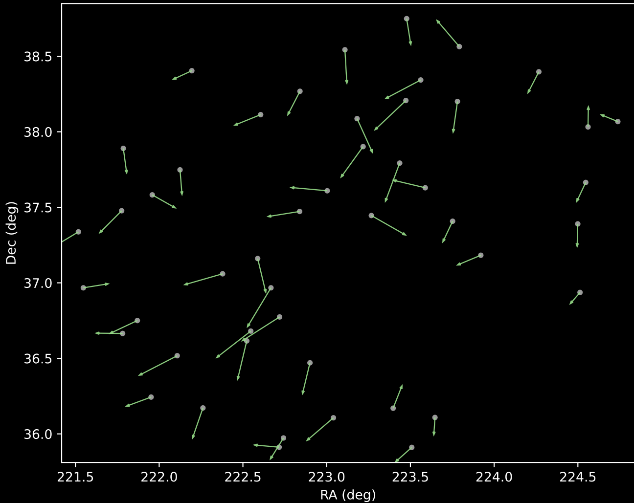
APOGEE DR17 Cluster 5 Proper Motion Vectors (n=48)
